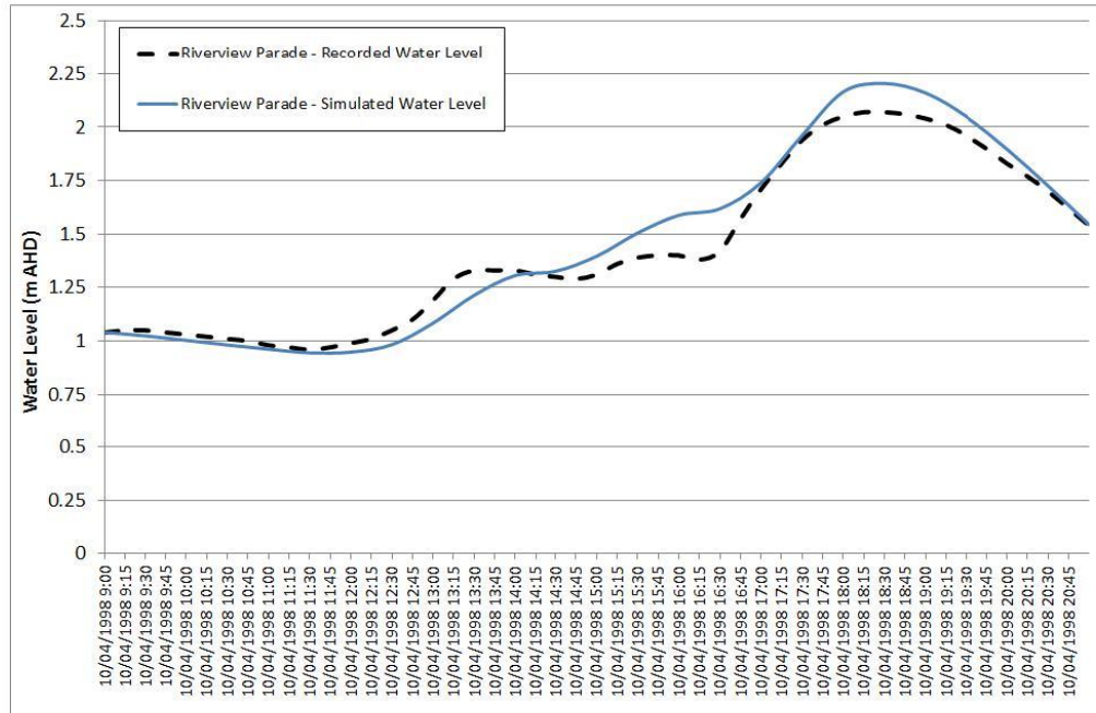
Figure 5-16 Riverview Parade Water Level Calibration – April 1998
