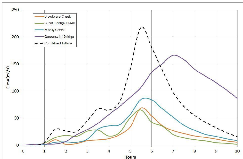
Figure 7-5 Sub-catchment Contributions to Manly Lagoon (1% AEP Event)
