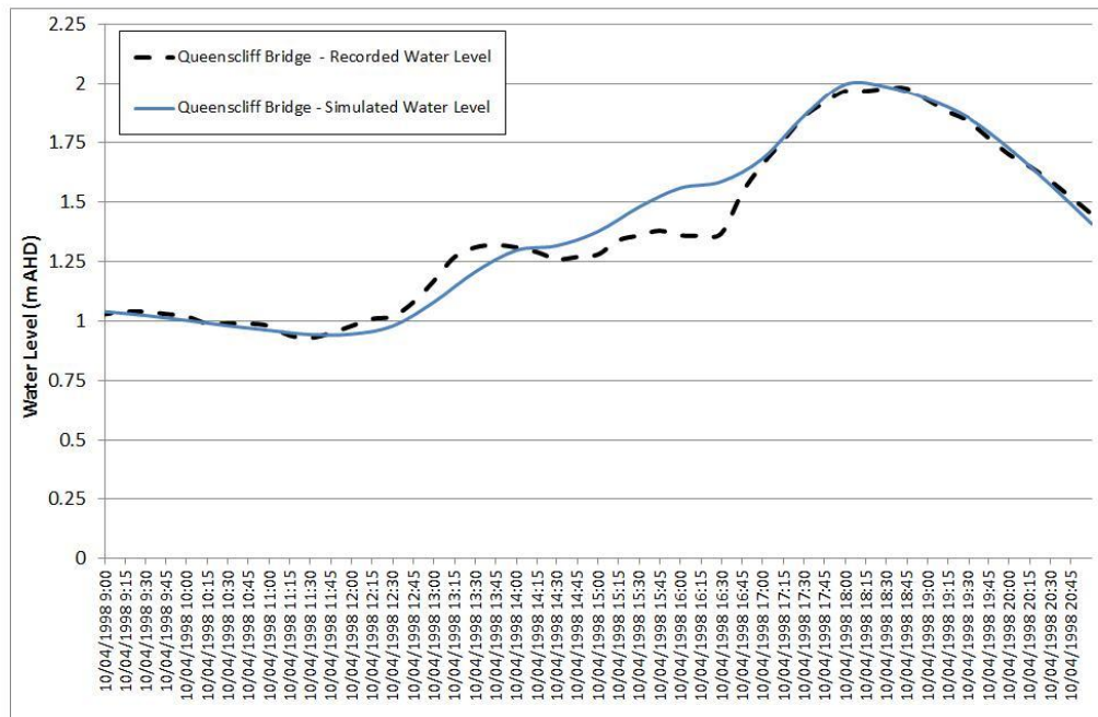
Figure 5-17 Queenscliff Bridge Water Level Calibration – April 1998
