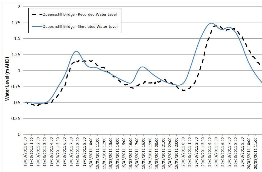
Figure 5-9 Queenscliff Bridge Water Level Calibration – March 2011
