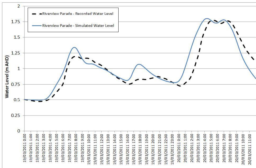
Figure 5-8 Riverview Parade Water Level Calibration – March 2011
