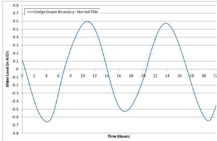
Figure 6-2 Design Ocean Boundary – Normal Tide
