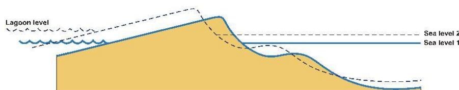
Figure 8-1 Shoreline response to increasing sea level (Hanslow et al. , 2000)
