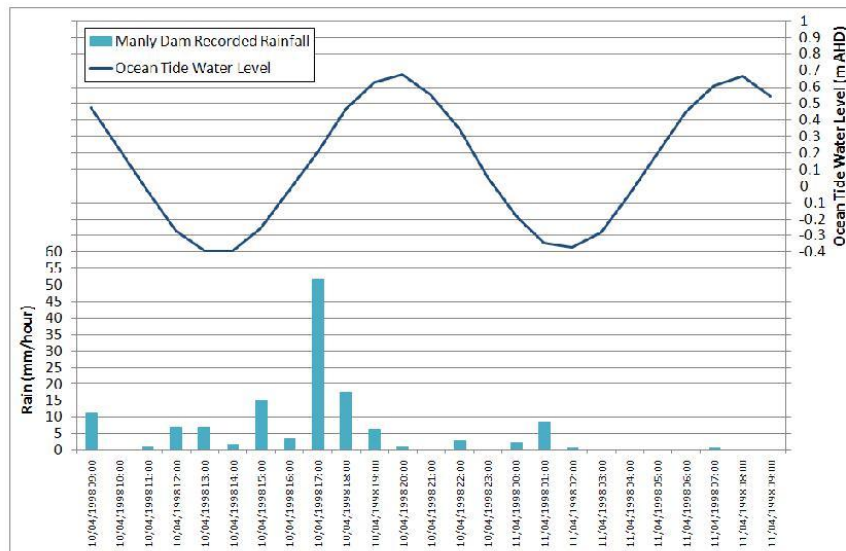
Figure 5-15 April 1998 Recorded Tidal Water Level
