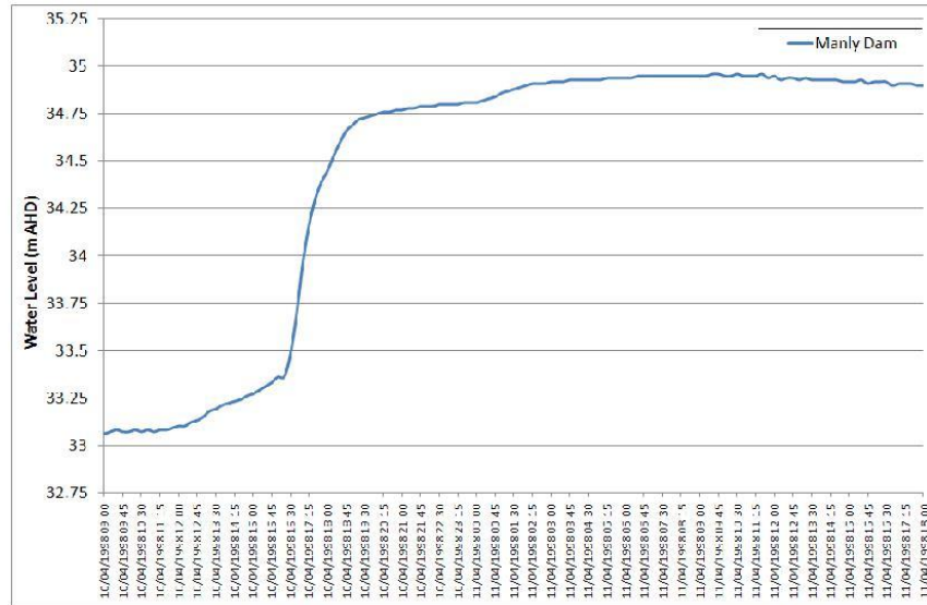
Figure 5-14 April 1998 Recorded Water Levels at Manly Dam
