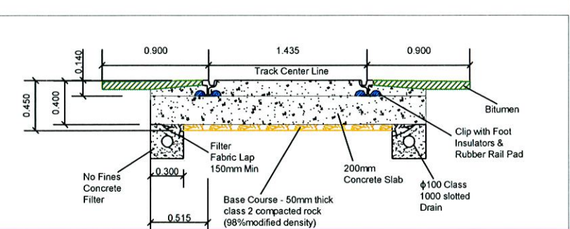
TRACK STRUCTURE - OPTION 3 FULL DEPTH CONCRETE TRACK SLAB WITHOUT STEEL BEAM
