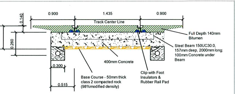
TRACK STRUCTURE - OPTION 2 FULL DEPTH BITUMEN - CONCRETE TRACK FOUNDATION WITH STEEL BEAM
