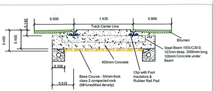
TRACK STRUCTURE - OPTION 1 FULL DEPTH CONCRETE TRACK SLAB WITH STEEL BEAM
